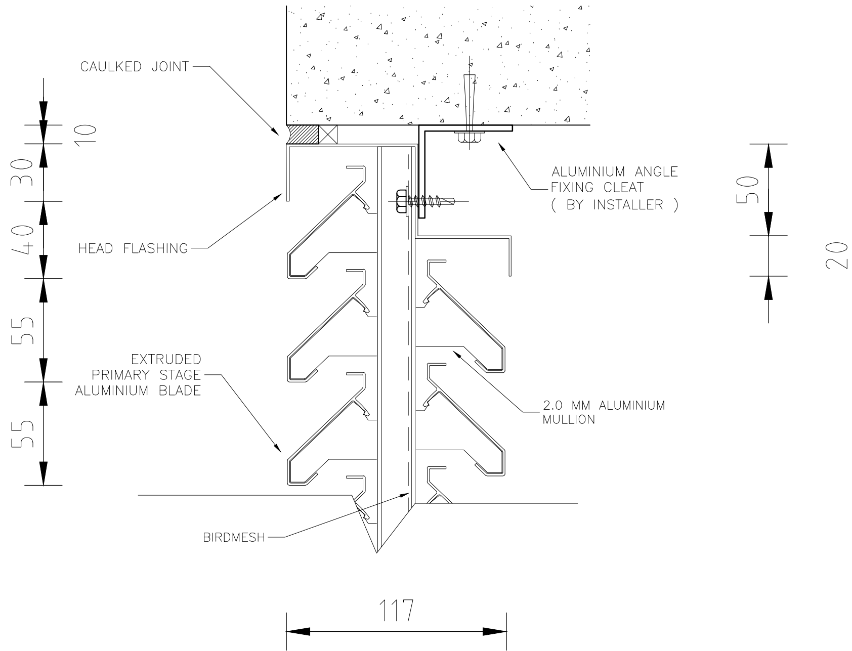
ELEMENT CONTROL SYSTEMS 55 DUAL STAGE LOUVRE HEAD INTO MASONRY
