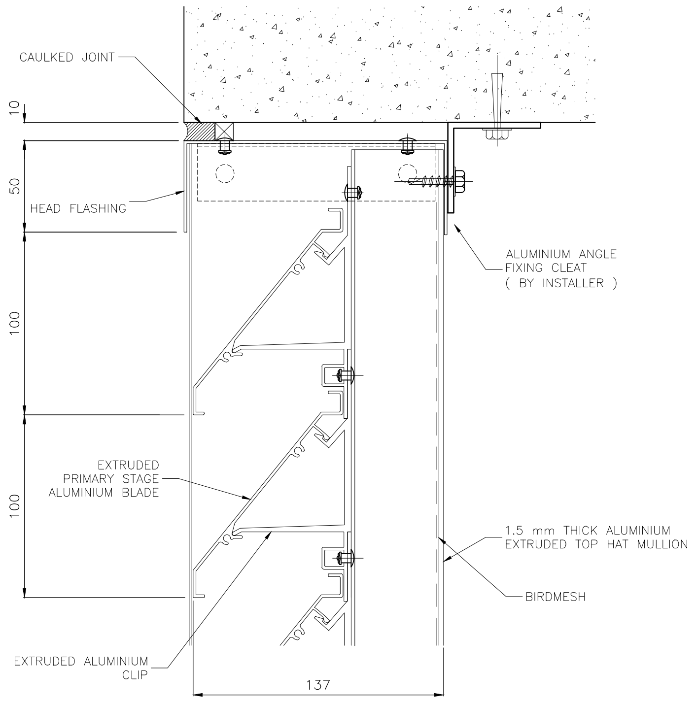
ELEMENT CONTROL SYSTEMS 100 PRIMARY STAGE LOUVRE HEAD INTO MASONRY
