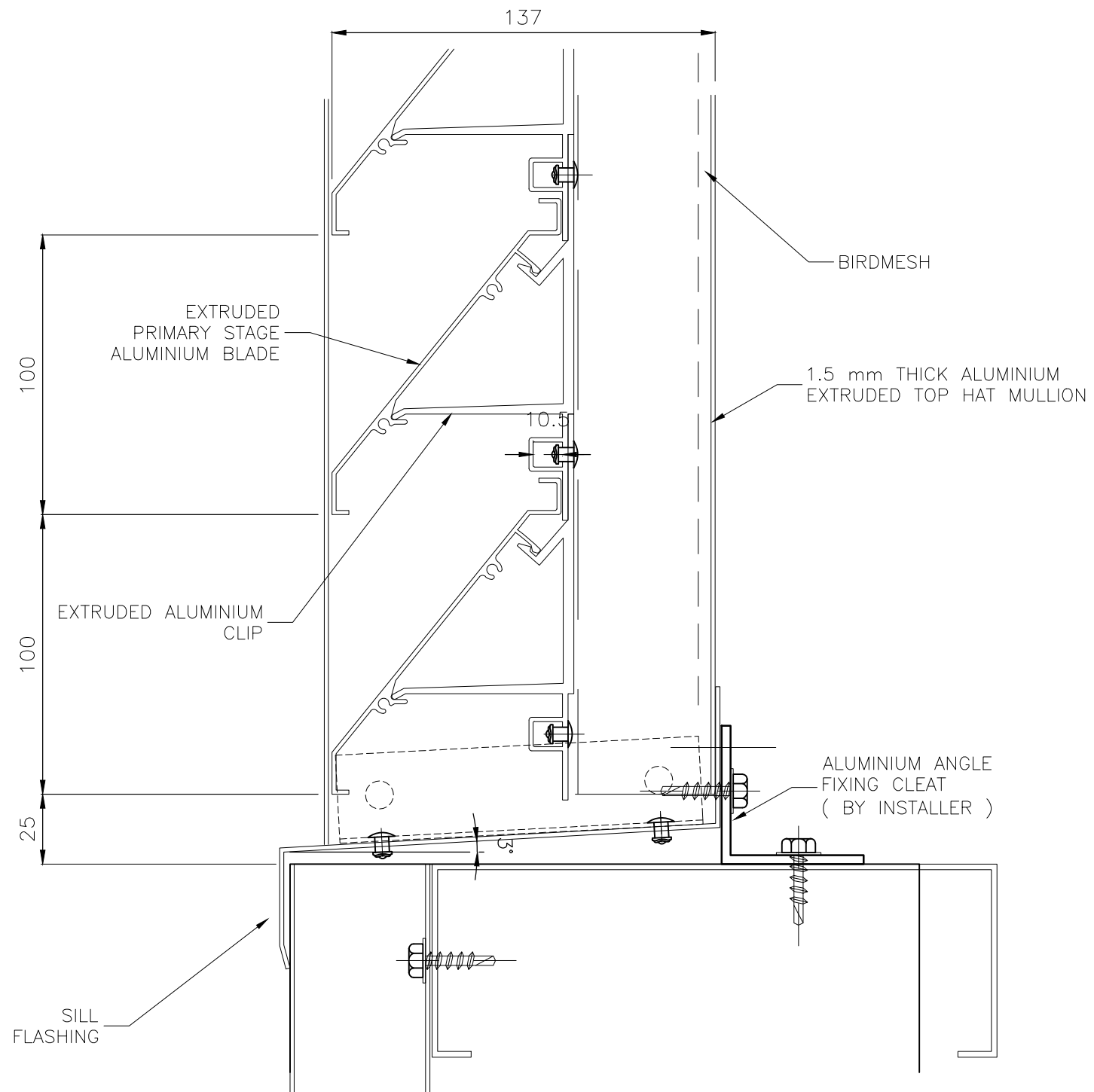
ELEMENT CONTROL SYSTEMS 100 PRIMARY STAGE LOUVRE SILL INTO CLADDING
